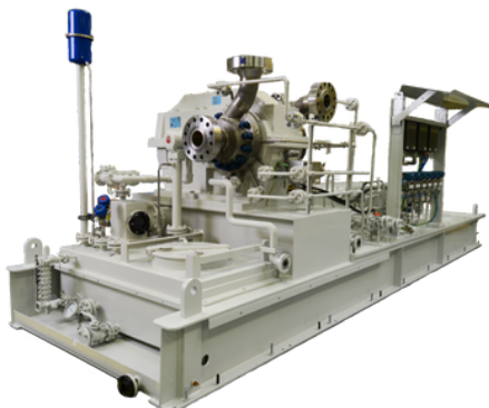
Urea Pump
