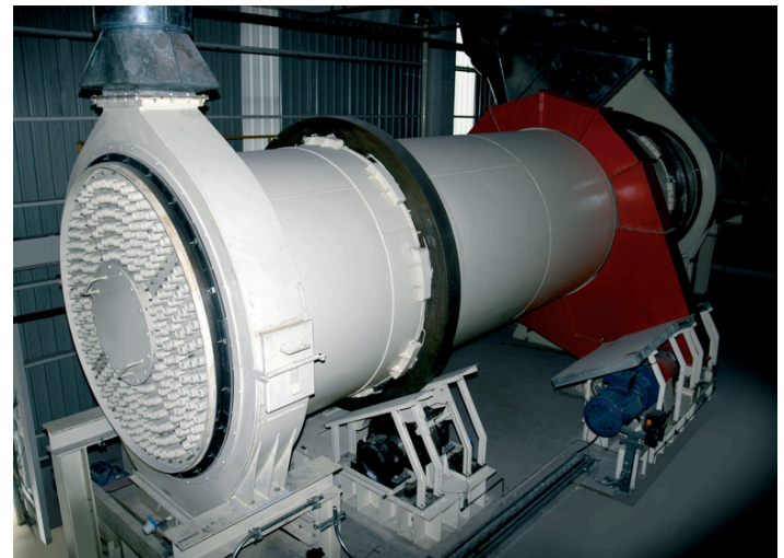
Rotary Drum Cooler for Calcined Gypsum
