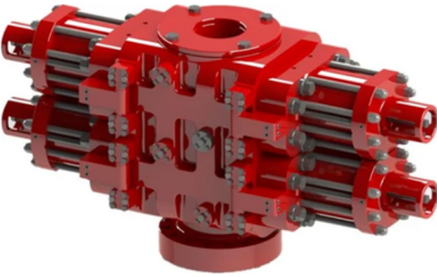
RAM type BOP
