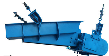
Electromagnetic Vibruator Feeder
